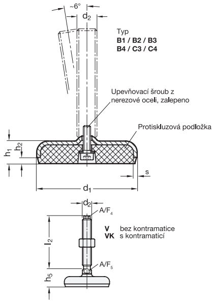
* Complete with version of Leveling feet (External hex socket on the top / Wrench flat at the bottom) V without nut VK with nut
